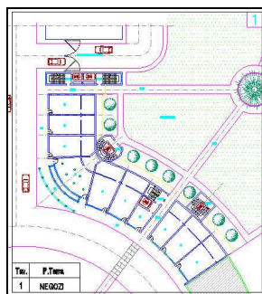
Piano terra
